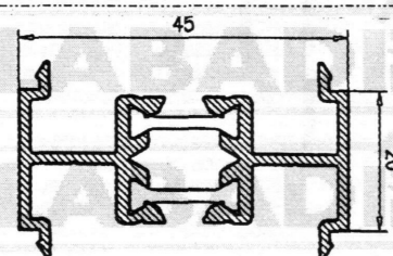
Union Marcos 54281
